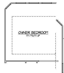
OPT. MASTER BAY
