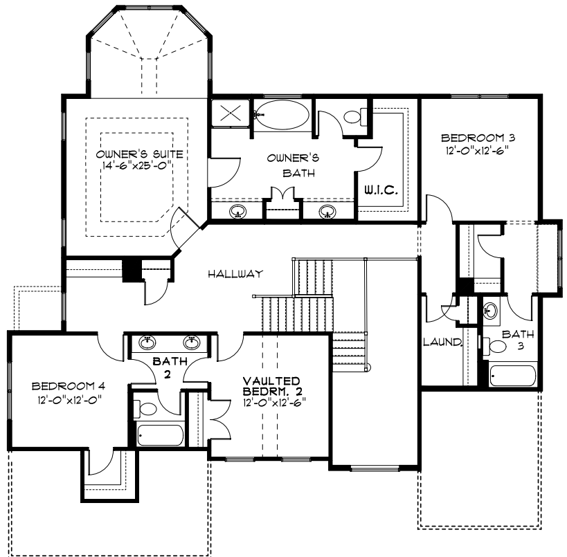
SECOND FLOOR
